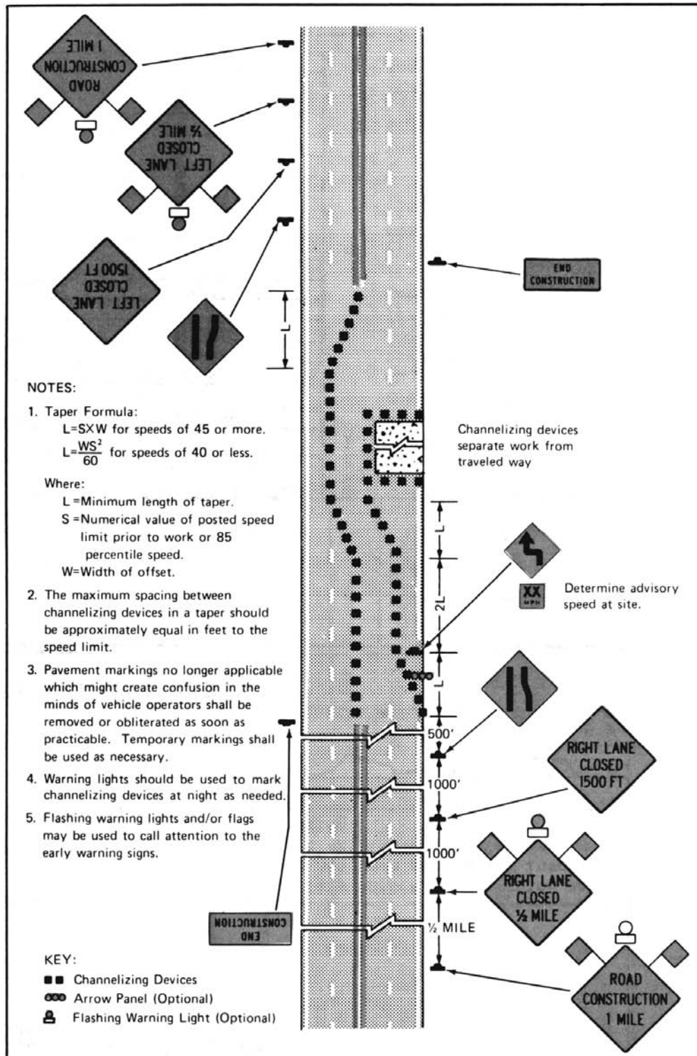
Figure 6. The recommended arrangement of warning devices and barricades when a repair project closes half of a four lane undivided roadway.
