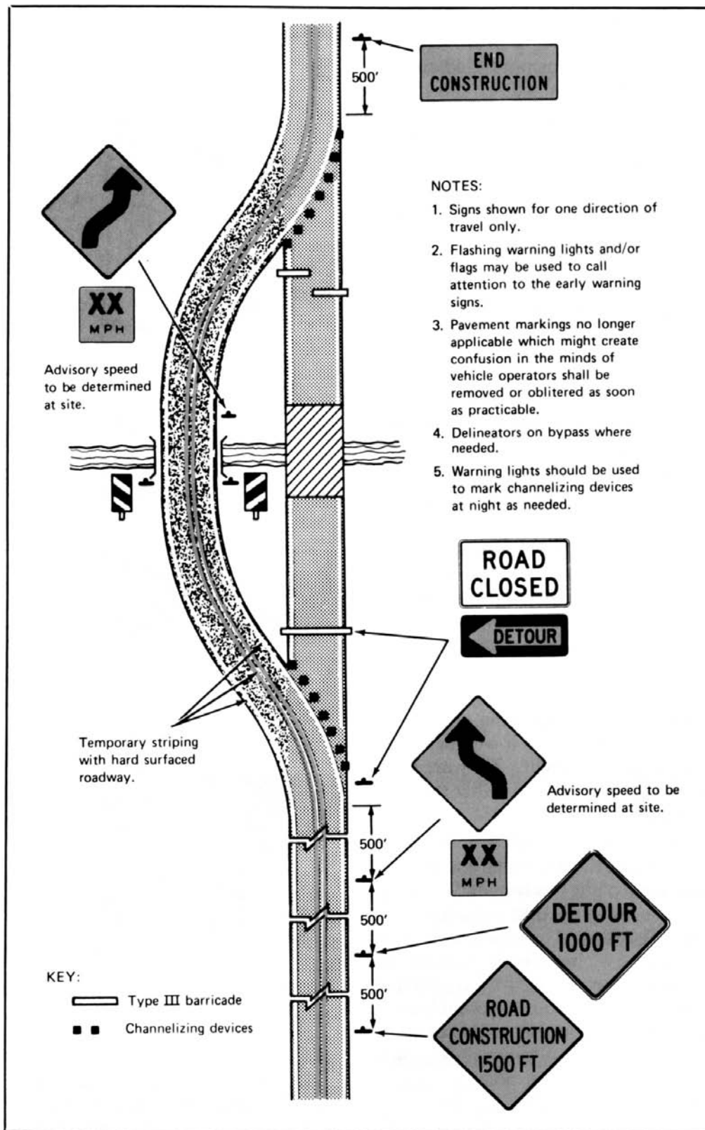
Figure 4. The recommended placement of various barricades and warning devices on a two-lane highway where the entire roadway is closed and a detour is provided.
