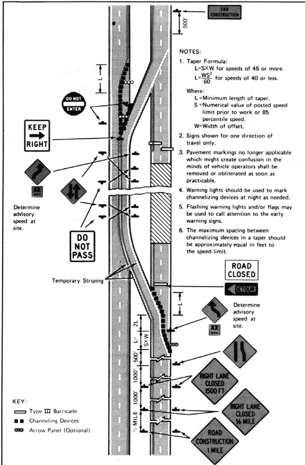
Figure 5. The recommended placement of various barricades and warning devices for construction or repair projects on four-lane divided roadway where one roadway is closed.
